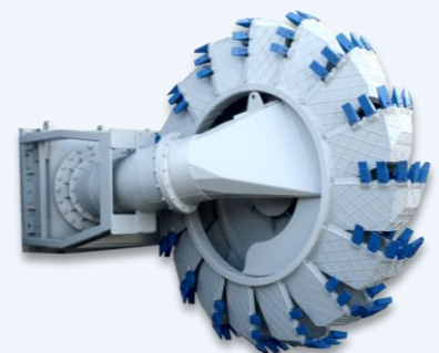
3500mm Dia. Dredge Bucketwheel Cutter and Suction Duct
