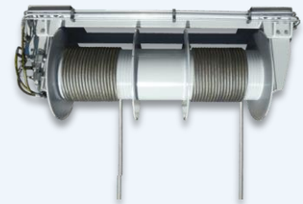
Overhead Gantry Style Hoist Winch
