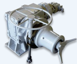
Single Side Gypsy Windlass (L) Anchor Winch
