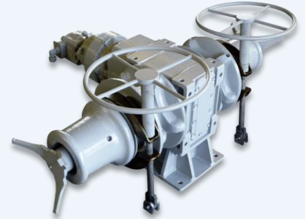
Double Sided Gypsy Windlass Anchor Winch
